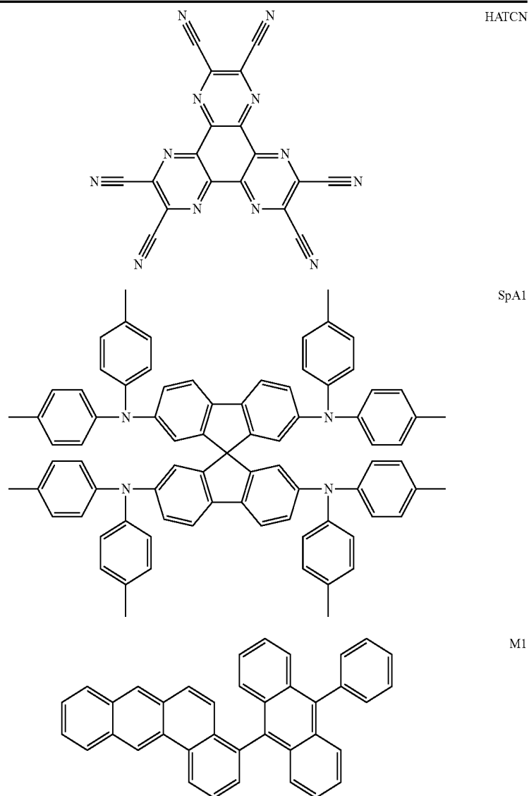
Structural formulae of the materials for the OLEDs
